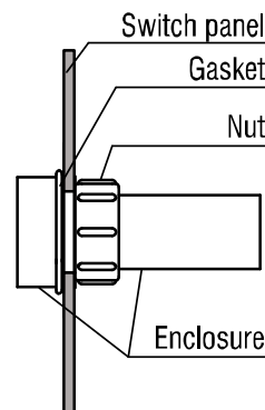
Fig. 5.4 Mounting
